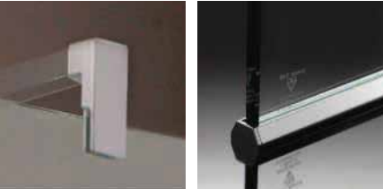
Bracing bar detail Silicone free sealing membrane suitable for tray or floor tiles
