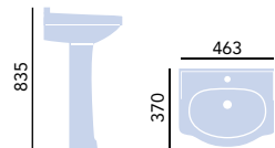
Cloakroom Basin & Pedestal PRHW071 1 Taphole Basin £95 PRHW07 2 Taphole Basin £95 PRHW09 Pedestal £72
